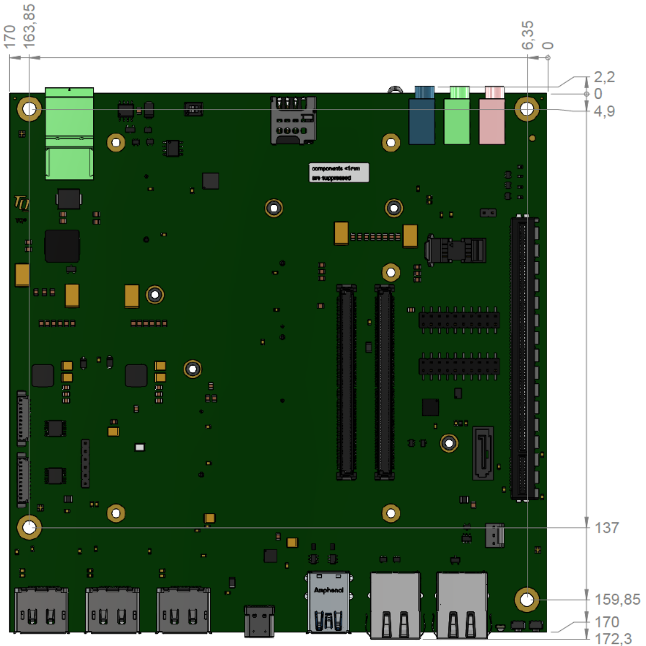
Figure 14: MB-COME6-4 Dimensions
