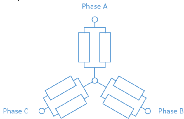
Star-parallel
