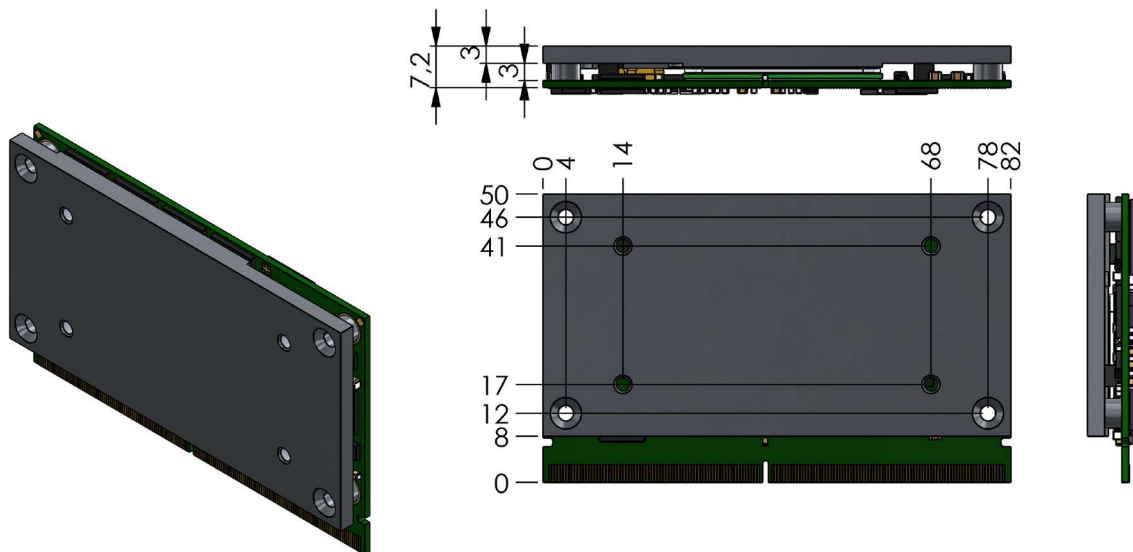
Figure 3: Standard Heat Spreader TQMxE41S-HSP (dimensions in mm)
