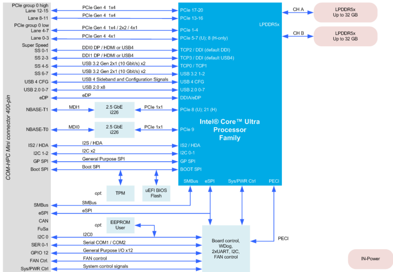
Figure 1: TQMxCU1-HPCM Block Diagram
