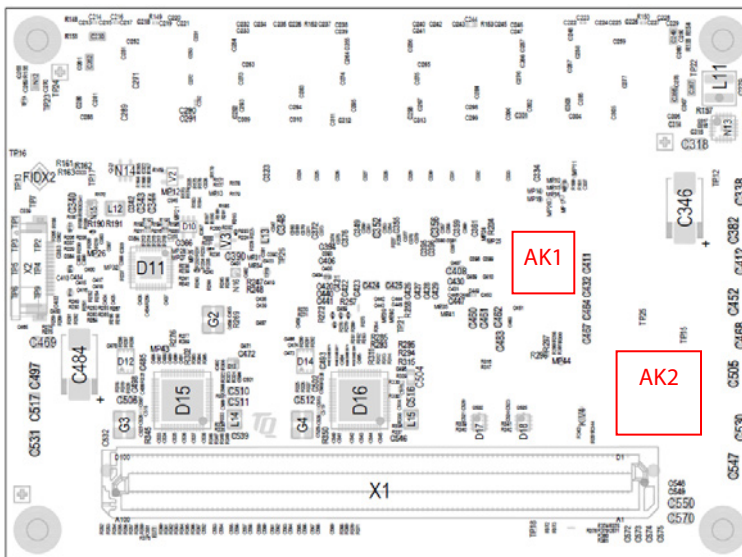
Figure 8: TQMxCU1-HPCM Component Placement Bottom
