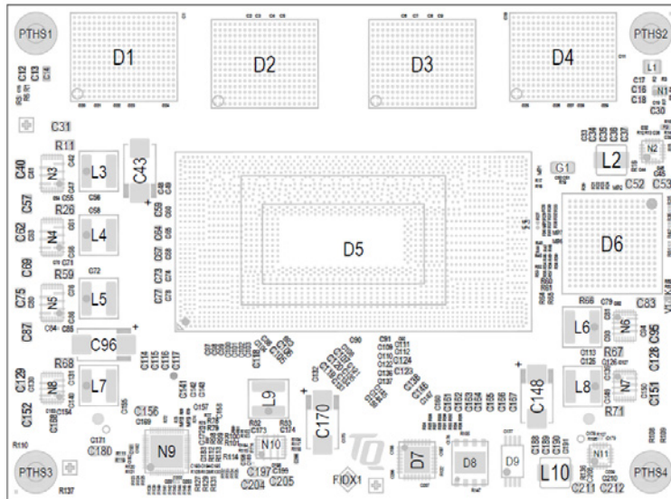
Figure 7: TQMxCU1-HPCM Component Placement Top
