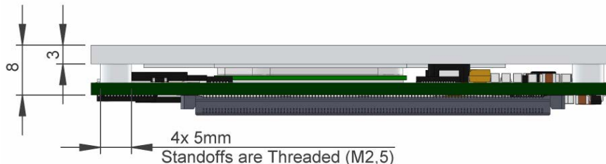
Figure 5: Low-Profile Heat Spreader TQMxE39M-HSP-LP
