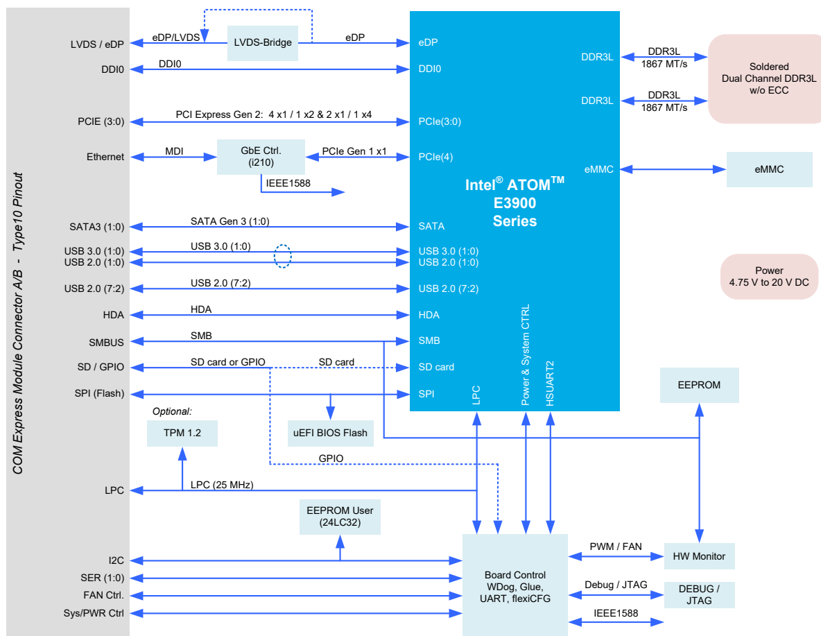
Figure 1: Block Diagram TQMxE39M
