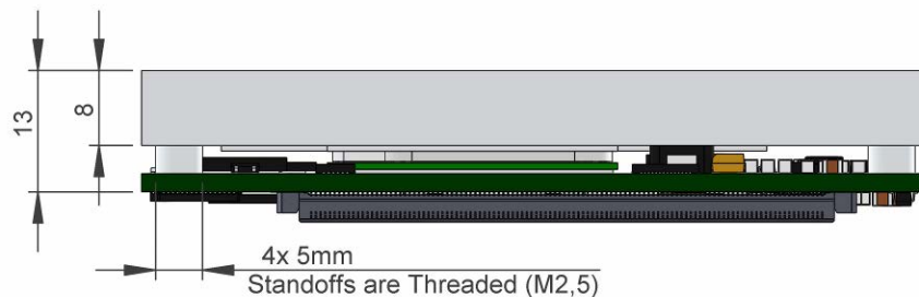
Figure 4: Standard Heat Spreader TQMxE39M-HSP
