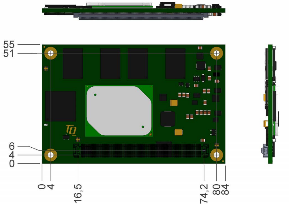
Figure 2: Three view drawing TQMxE39M
