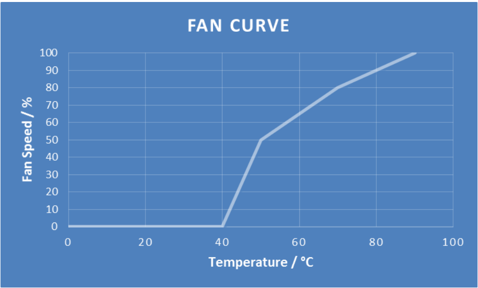
Figure 7: Fan Curve
