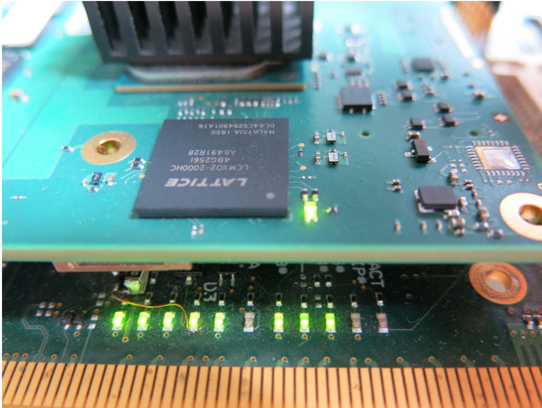
Illustration 12: TQMxE39C2 Debug LED
