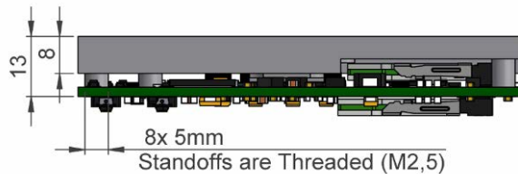
Illustration 7: TQMx80UC-HSP Heat Spreader
