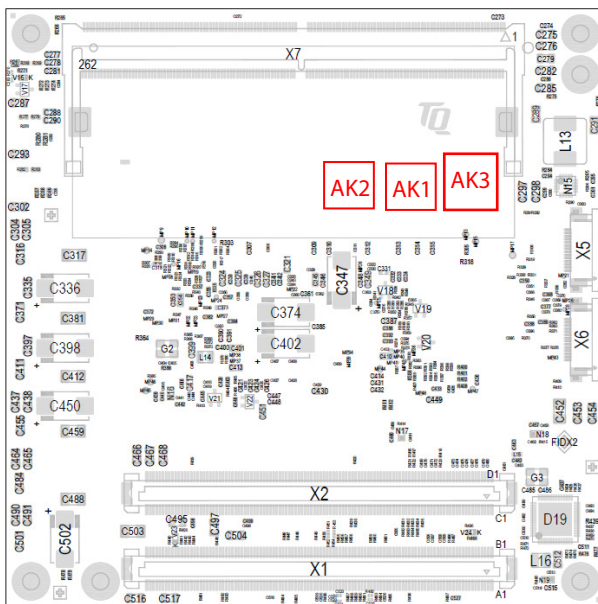
Figure 7: TQMx130 Component Placement Bottom
