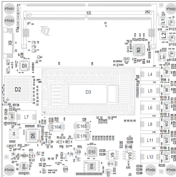
Figure 6: TQMx130 Component Placement Top
