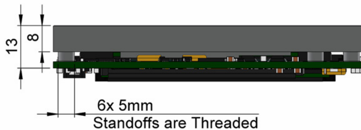
Figure 8: TQMx130-HSP Heat Spreader
