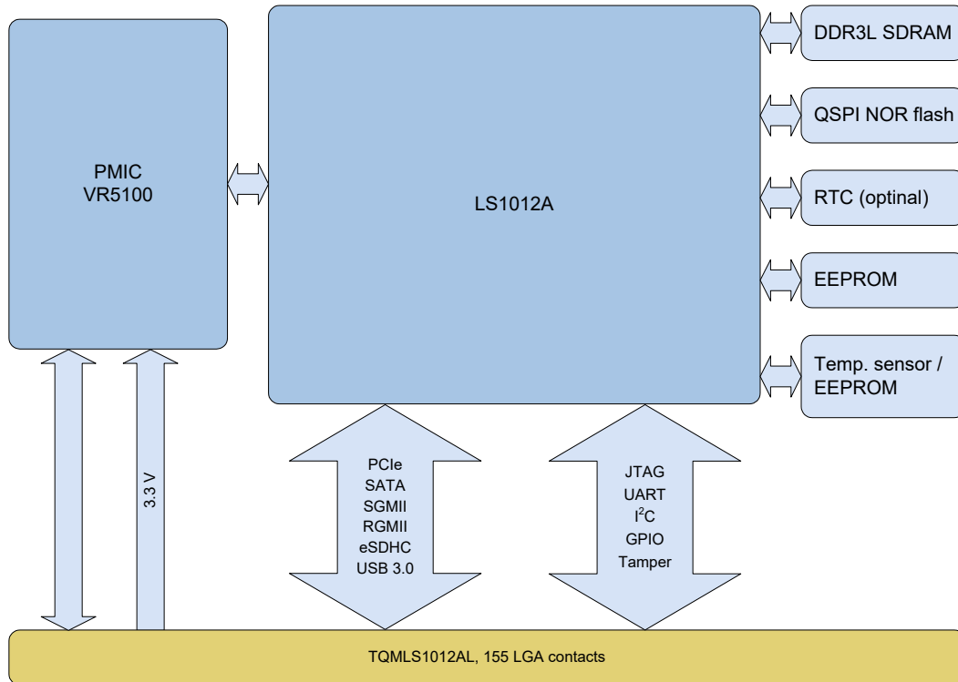
Figure 2: Block diagram TQMLS1012AL (simplified)
