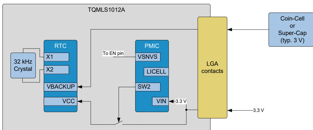
Figure 4: Block diagram RTC
