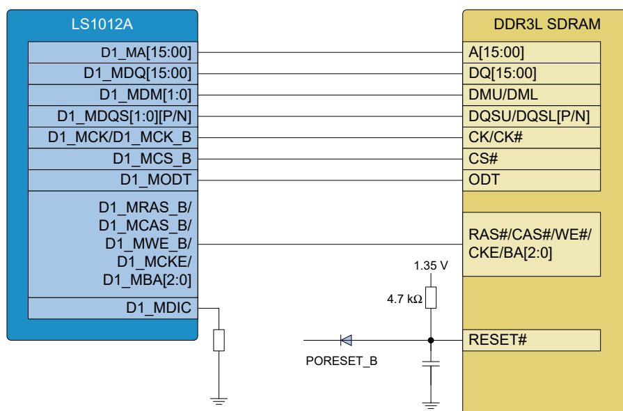
Figure 3: TQMLS1012AL DDR3L SDRAM interface
