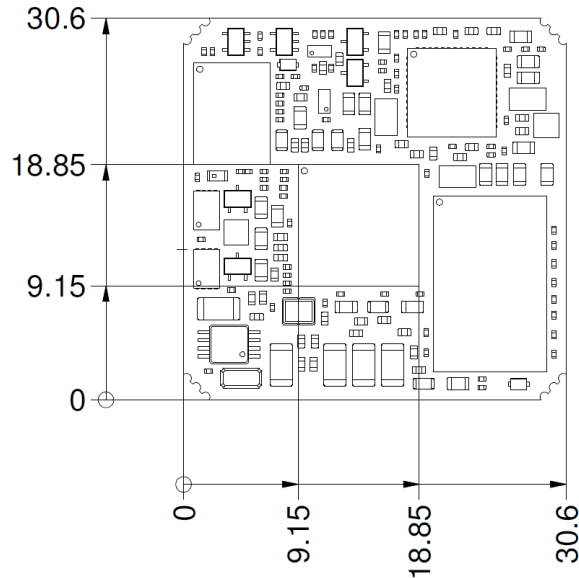
Figure 8: TQMLS1012AL dimensions, top view
