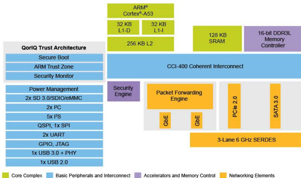
Figure 1: Block diagram LS1012A (Source: NXP )
