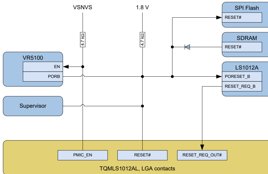
Figure 5: Block diagram Reset
