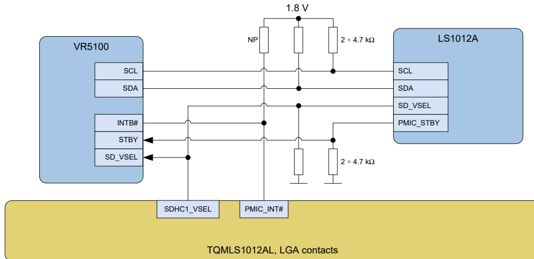
Figure 6: Block diagram PMIC interface
