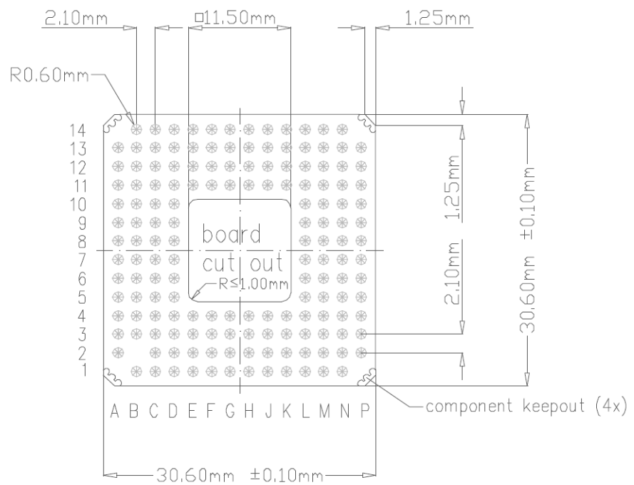
Figure 9: TQMLS1012AL dimensions, recommended PCB land pattern, top view through TQMLS1012AL
