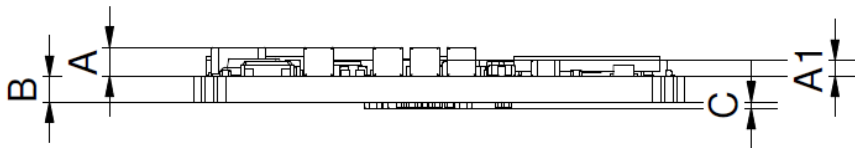
Figure 7: TQMLS1012AL dimensions, side view
