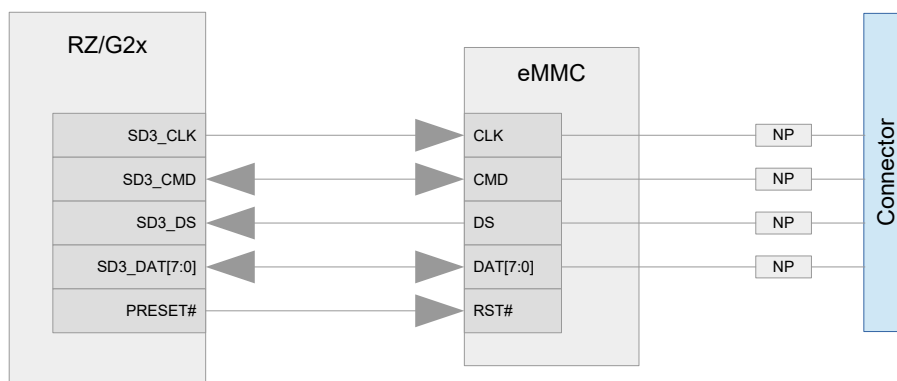
Figure 6: Block diagram eMMC interface
