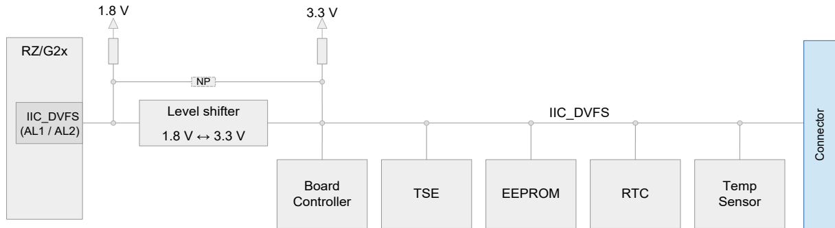
Figure 10: Block diagram I 2 C bus
