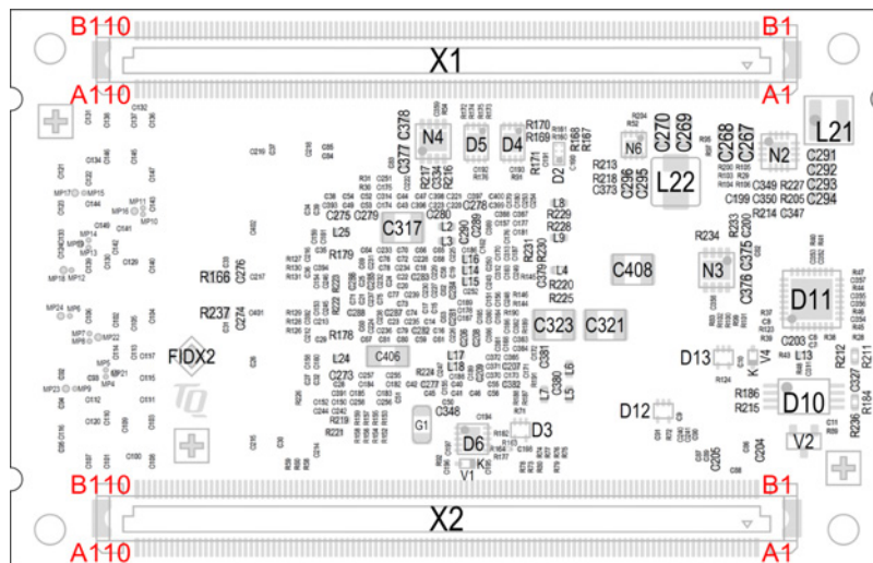
Figure 15: TQMaRZG2x assembly, bottom
