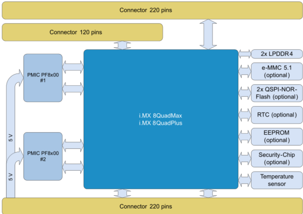
Figure 2: Block diagram TQMa8x
