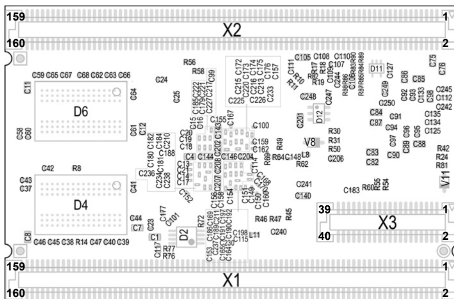
Figure 22: TQMa6x, component placement bottom
