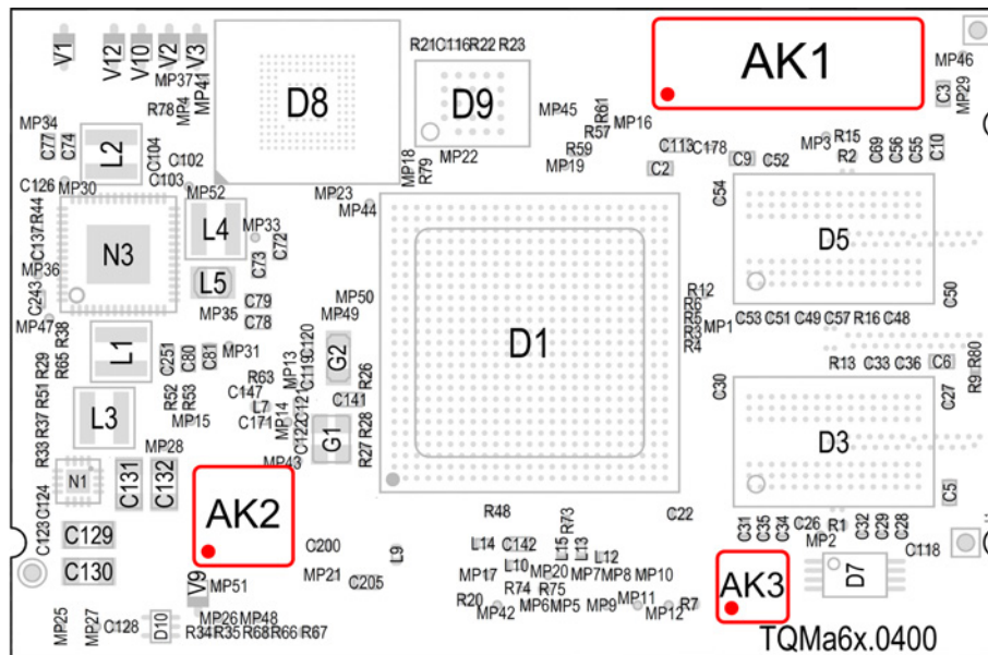
Figure 21: TQMa6x, component placement top
