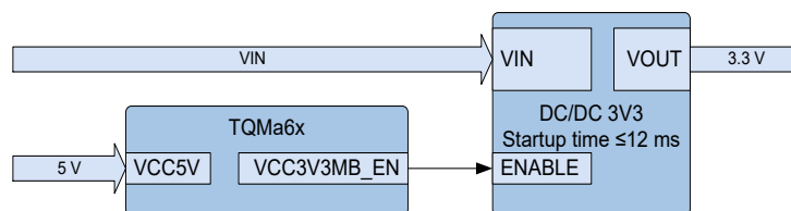
Figure 17: Block diagram power supply carrier board
