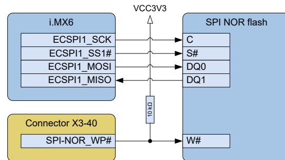
Figure 5: Block diagram SPI NOR flash connection
