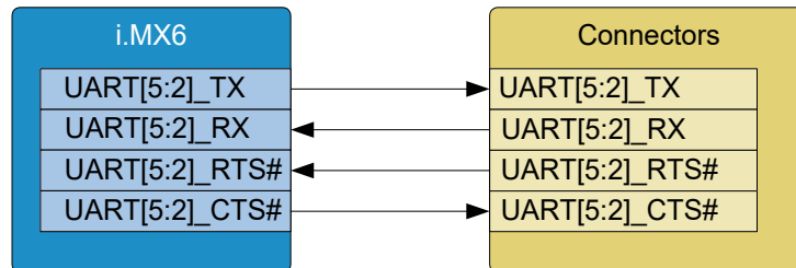
Figure 12: Block diagram UART interfaces
