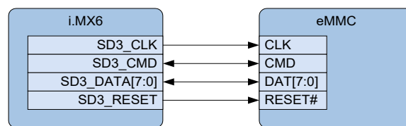
Figure 4: Block diagram eMMC NAND flash connection
