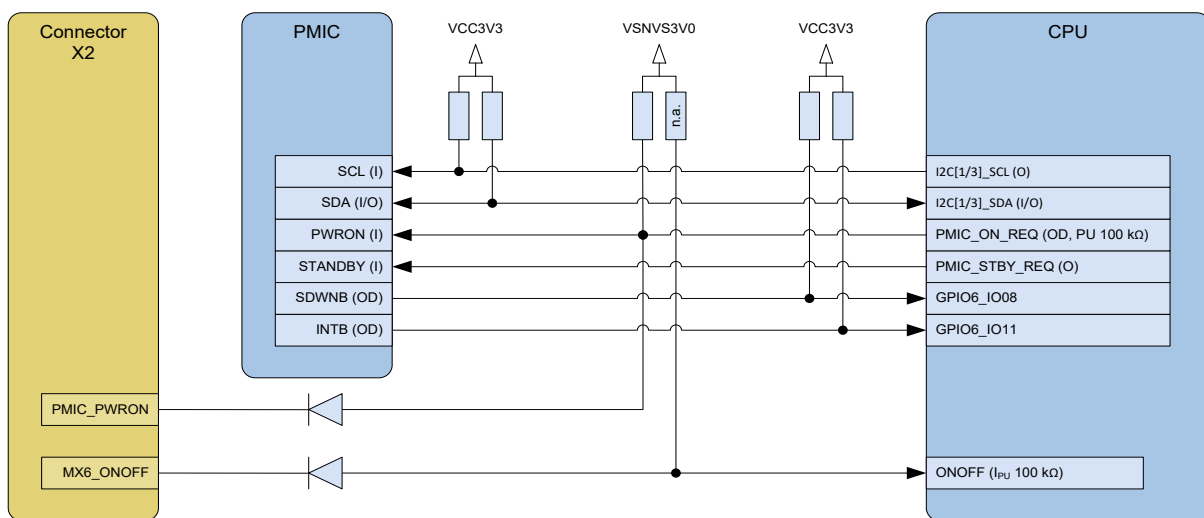
Figure 15: Block diagram PMIC signals
