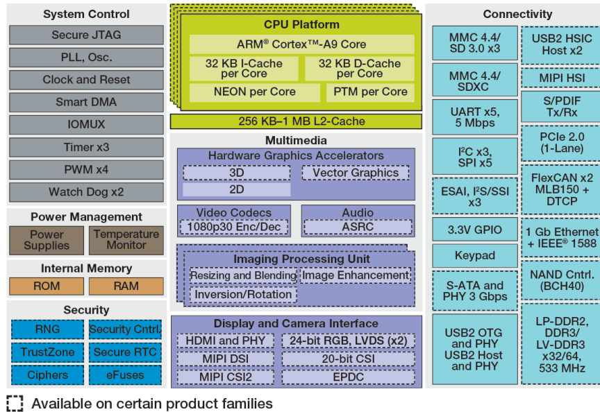
Figure 2: Block diagram i.MX6 (Source: NXP )
