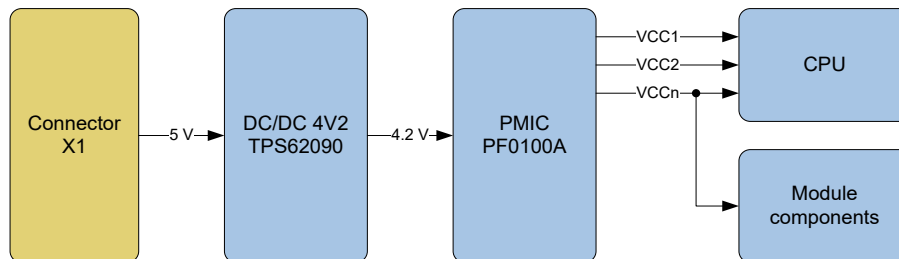
Figure 14: Block diagram power supply
