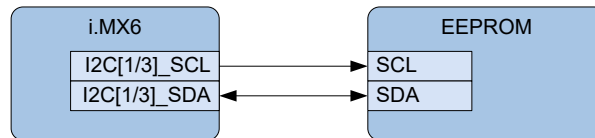
Figure 6: Block diagram EEPROM interface
