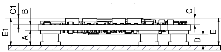
Figure 18: TQMa6x dimensions, side view
