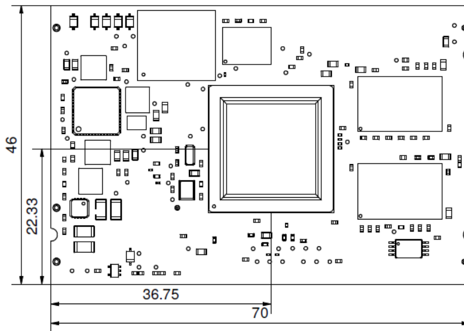
Figure 19: TQMa6x dimensions, top view
