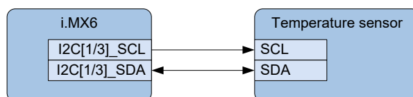
Figure 8: Block diagram temperature sensor interface
