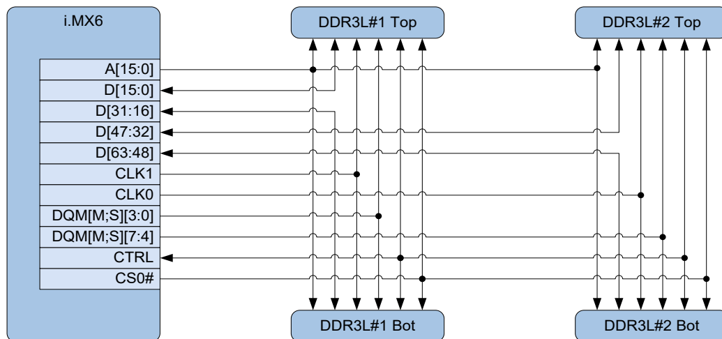
Figure 3: Block diagram DDR3L SDRAM connection
