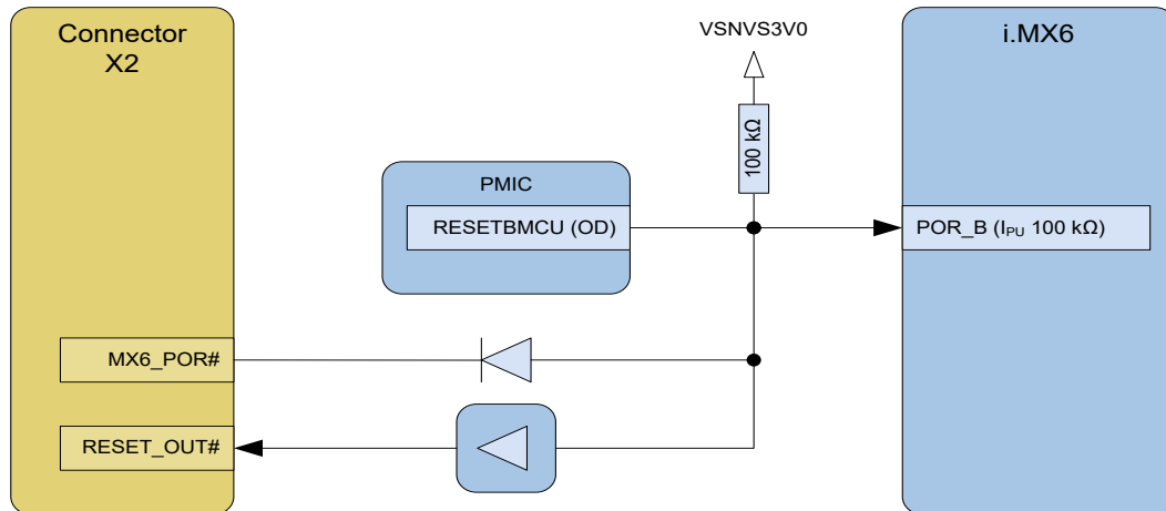
Figure 13: Block diagram Reset
