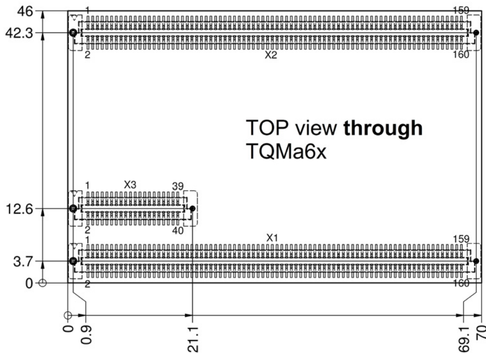
Figure 20: TQMa6x dimensions, top view through TQMa6x
