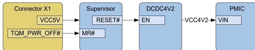
Figure 16: Block diagram VCC5V monitoring
