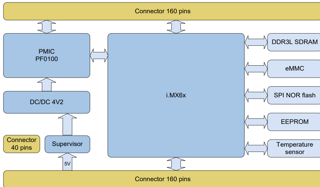
Figure 1: Block diagram TQMa6x
