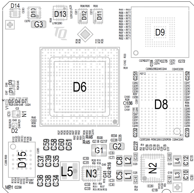
Figure 18: TQMa67xxL top view
