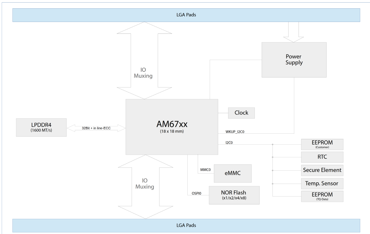
Figure 2: Block diagram TQMa67xxL
