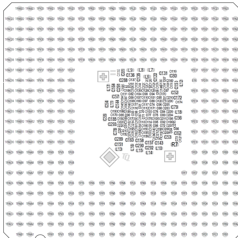
Figure 19: TQMa67xxL bottom view
