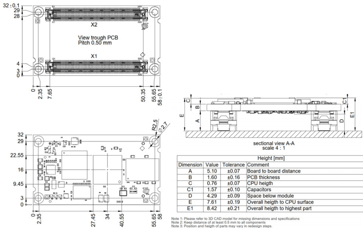
Figure 15: Dimensions
