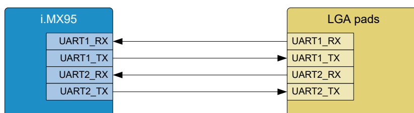
Figure 16: Block diagram UART
