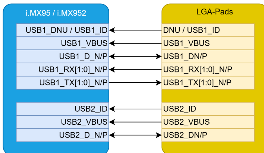
Figure 10: Block diagram USB
