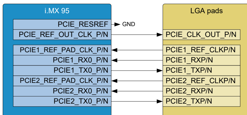
Figure 17: Block diagram PCI Express
