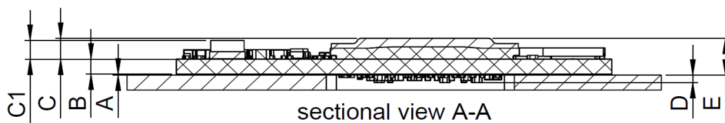
Figure 25: TQMa95xxLA heights with heatspreader
