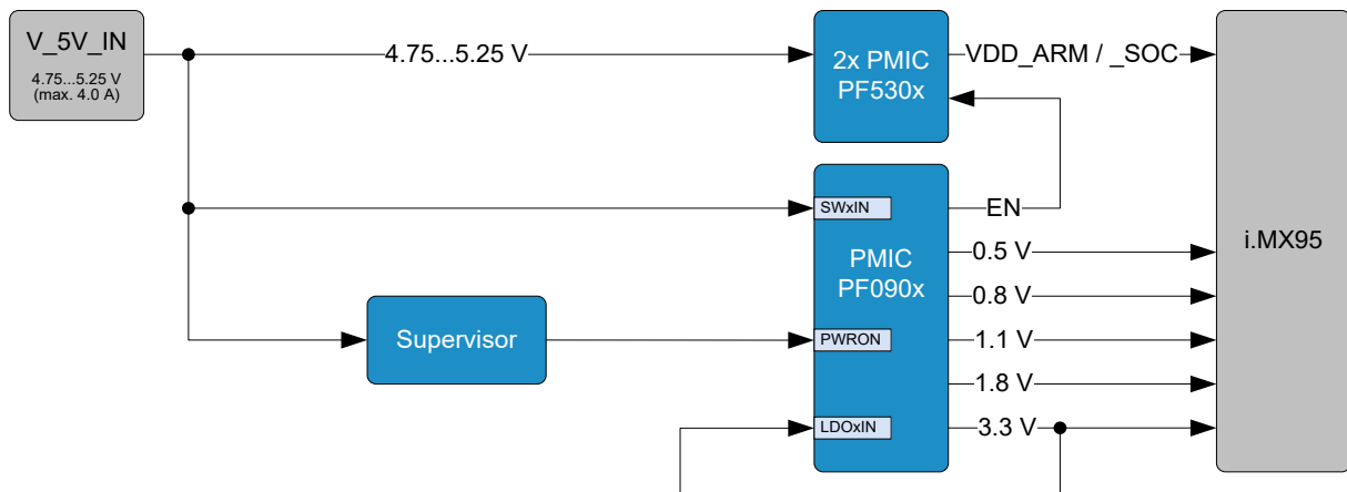
Figure 22: Block diagram module supply
