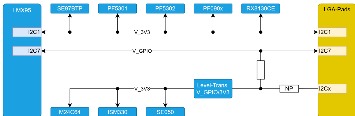
Figure 18: Block diagram I 2 C
