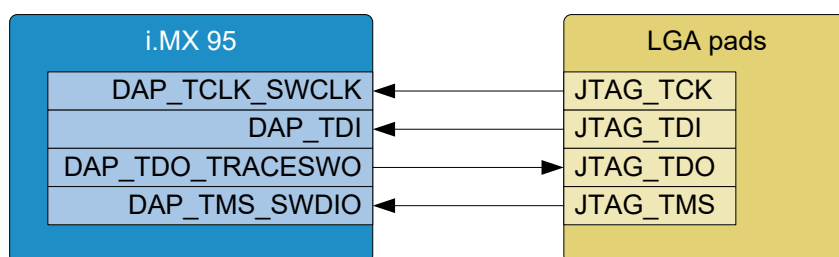
Figure 20: Block diagram JTAG
