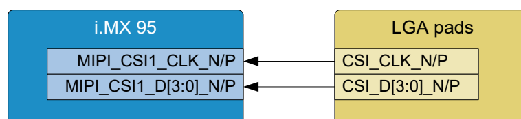
Figure 12: Block diagram CSI
