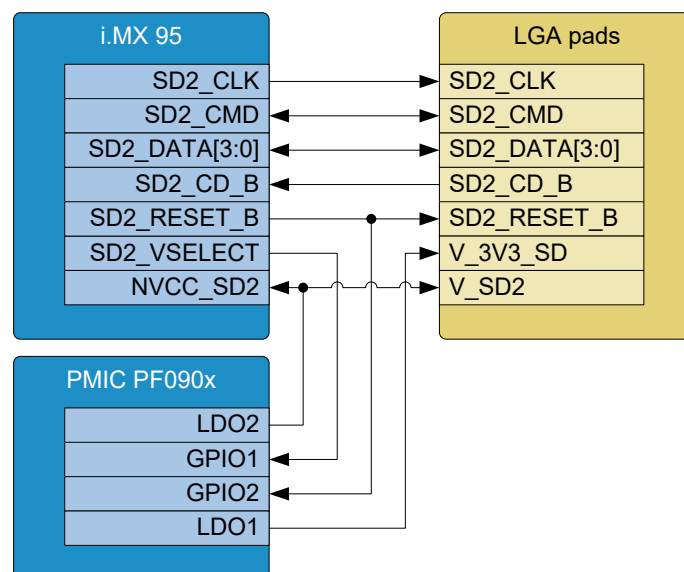
Figure 5: Block diagram SD Card
