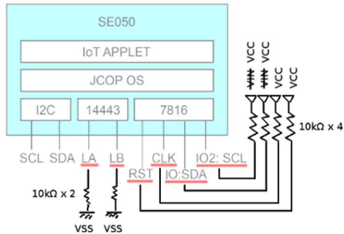
Figure 21: Connecting the NC-Pins (Source: NXP )
