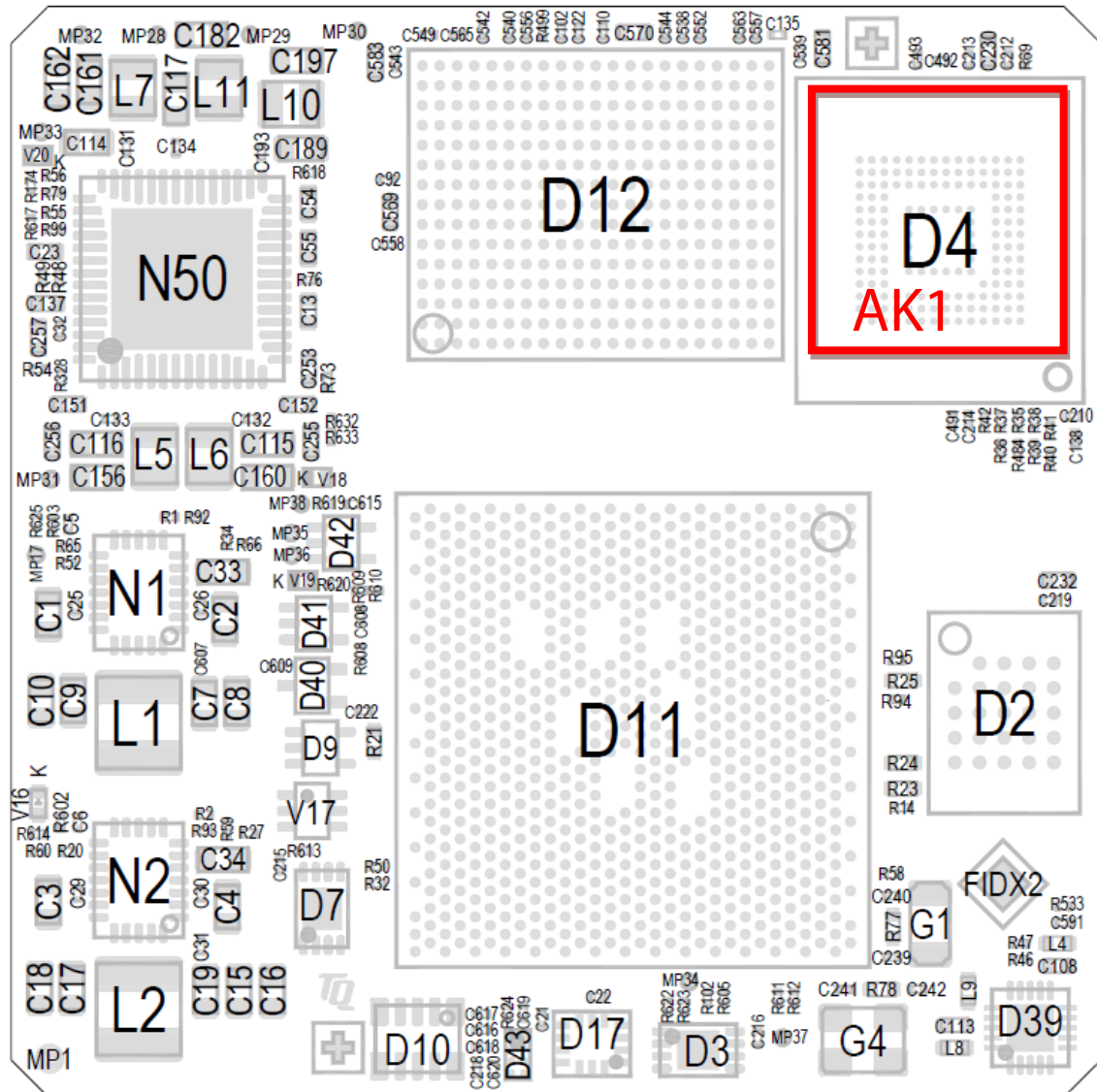
Figure 27: TQMa95xxLA, component placement top
