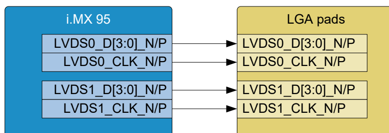
Figure 11: Block diagram LVDS
