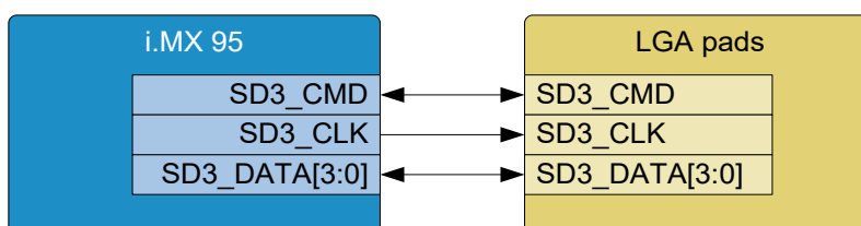
Figure 6: Block diagram USDHC3
