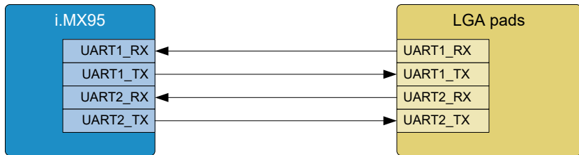
Figure 16: Block diagram UART
