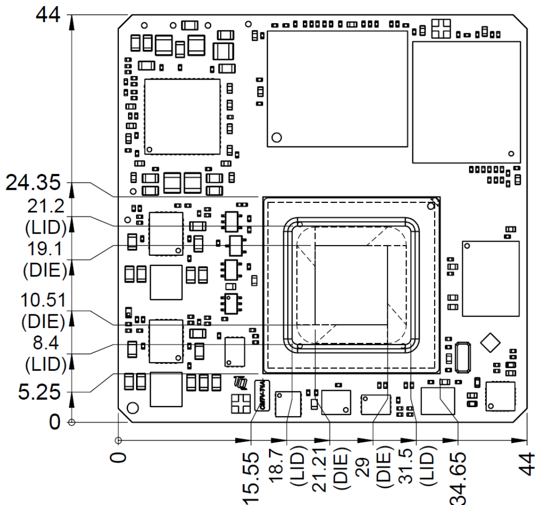
Figure 24: TQMa95xxLA dimensions (top view)
