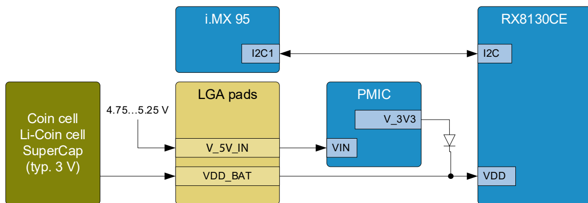
Figure 7: Block diagram RTC supply (TQMa95xxLA with discrete RTC)
