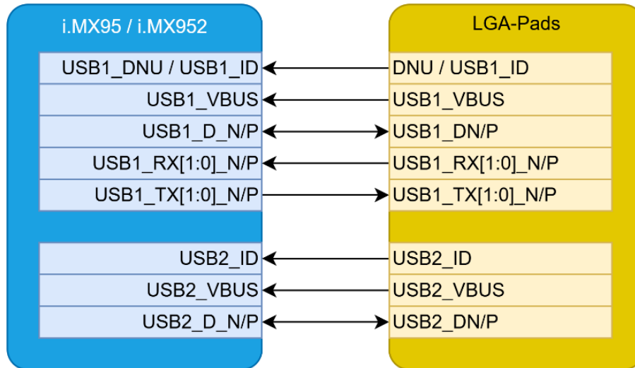
Figure 10: Block diagram USB
