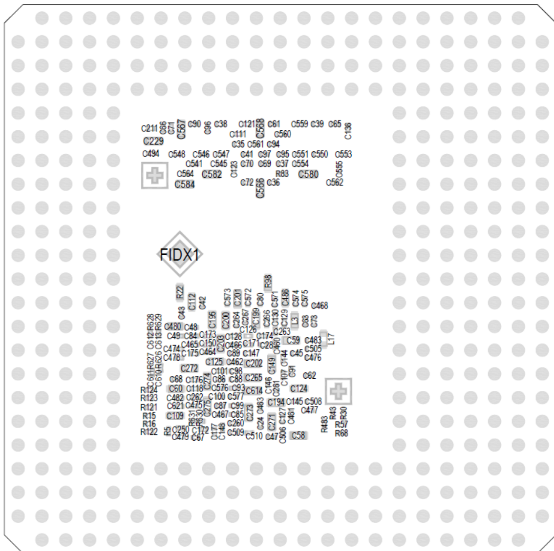
Figure 28: TQMa95xxLA, component placement bottom
