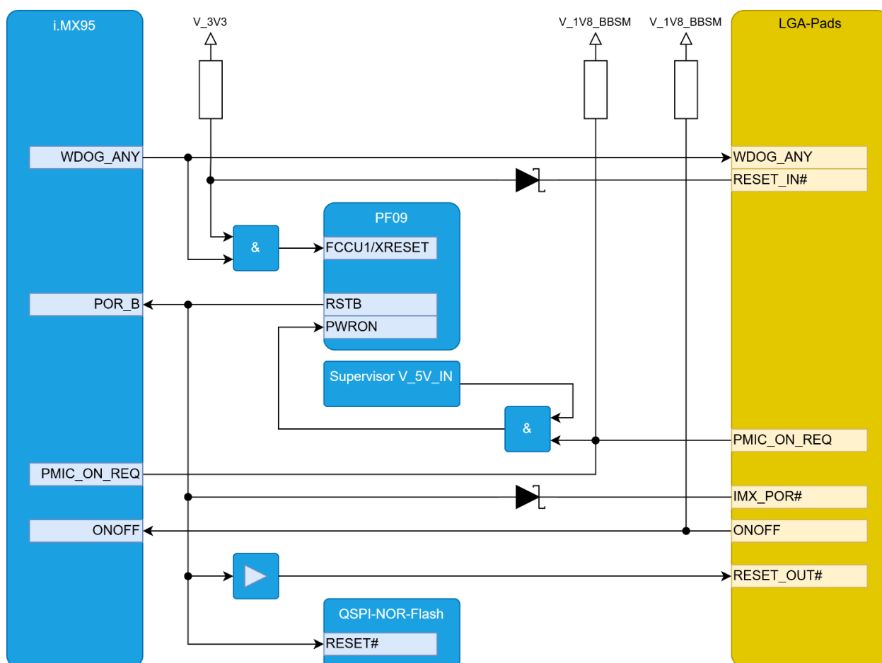
Figure 23: Block diagram Reset
