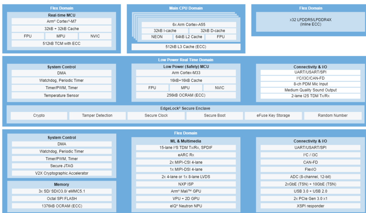
Figure 1: Block diagram i.MX 95 CPU
