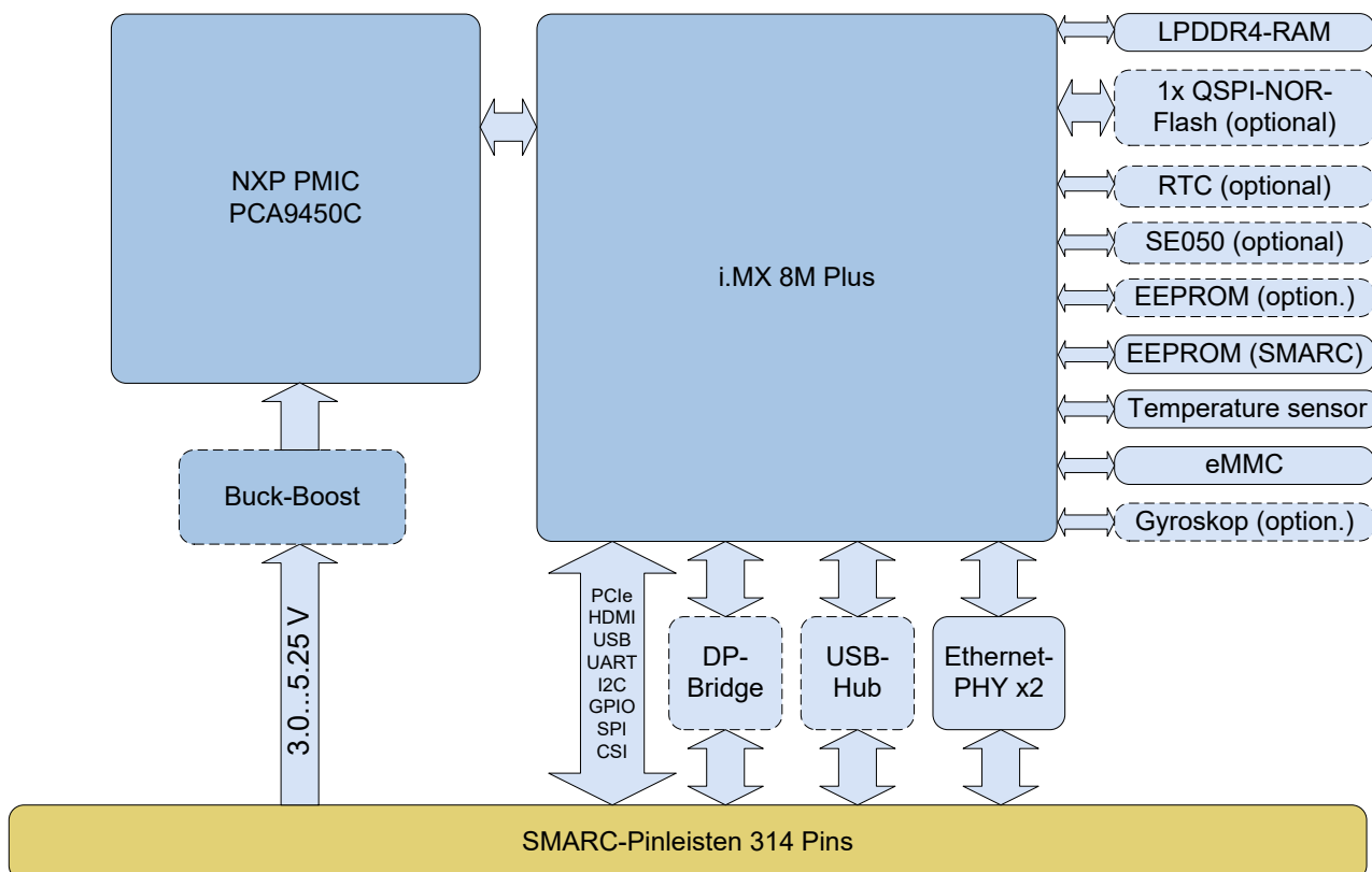
Figure 2: Block diagram TQMa8MPxS (simplified)
