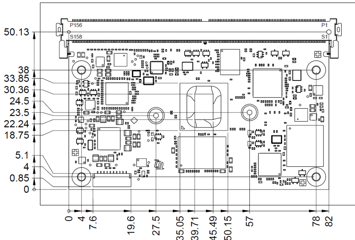
Figure 25: TQMa8MPxS dimensions (without heatspreader)
