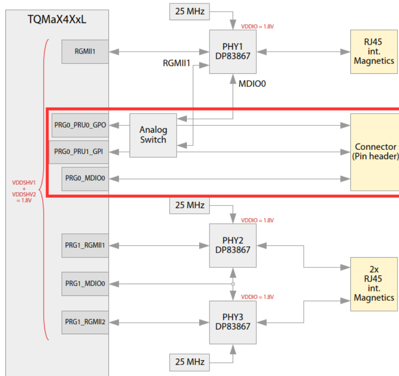
Figure 23: Block diagram PRU
