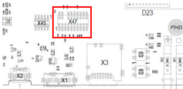
Figure 26: Position of JTAG, X47
