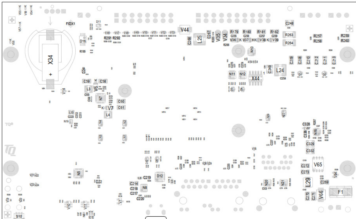
Figure 42: MBaX4XxL, component placement bottom
