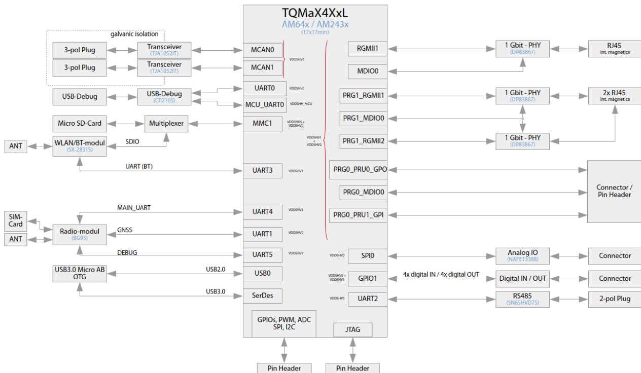
Figure 1: Block diagram MBaX4XxL
