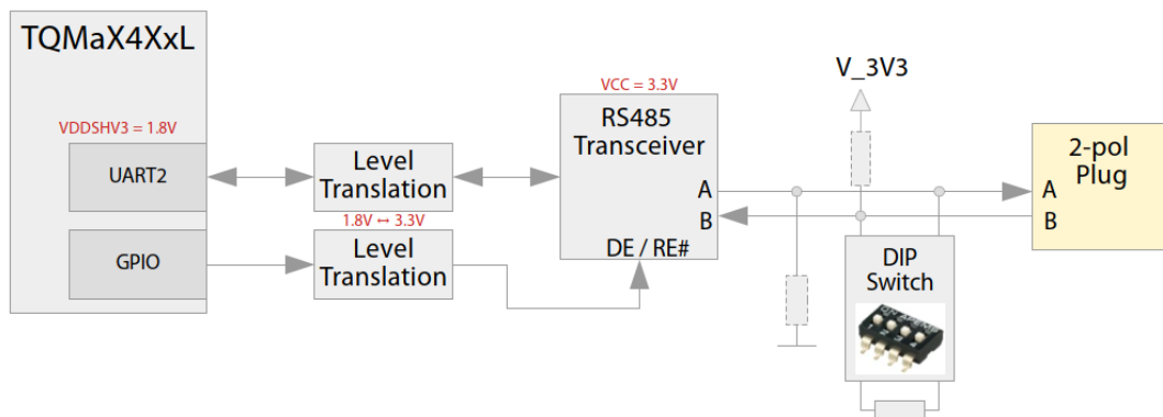
Figure 16: Block diagram RS485
