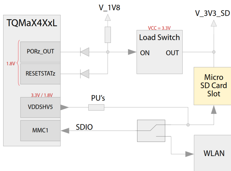
Figure 22: Block diagram SD card slot, X3
