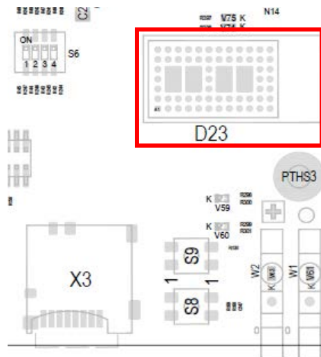
Figure 19: Position WLAN / WPAN module
