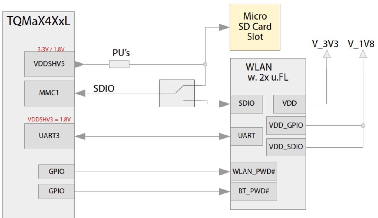
Figure 18: Block diagram WLAN / WPAN module
