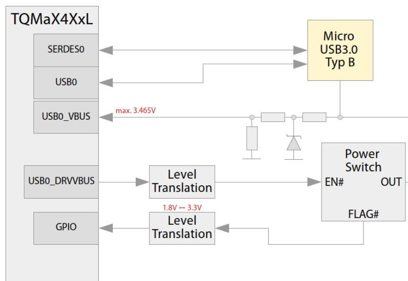
Figure 10: Block diagram USB interface
