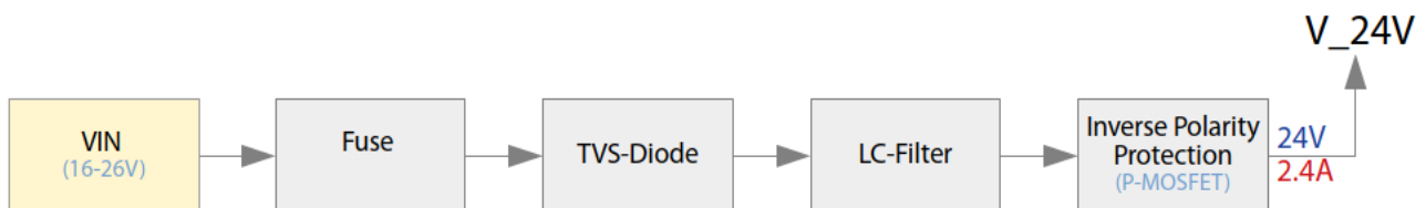
Figure 6: MBaX4XxL Input circuit
