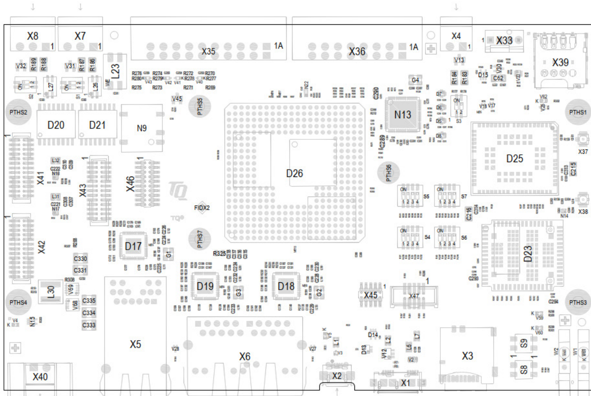
Figure 41: MBaX4XxL, component placement top
