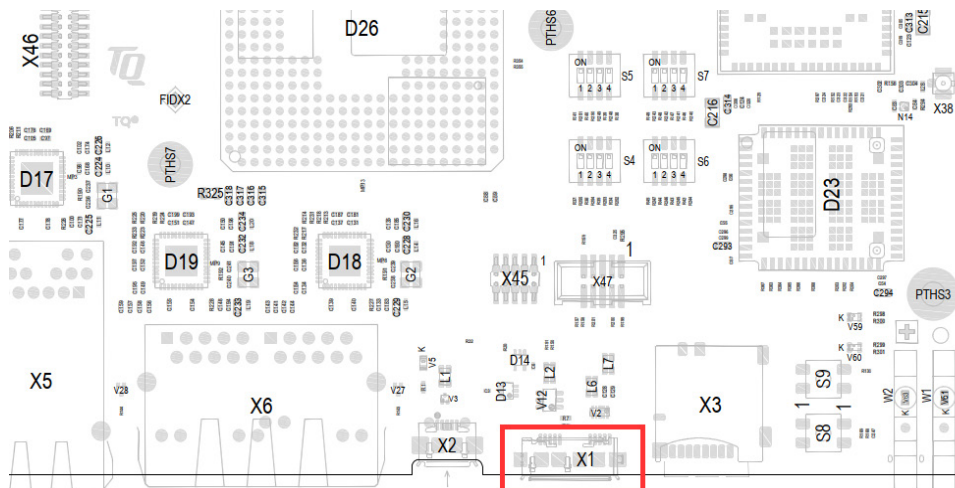
Figure 11: Position of USB interface
