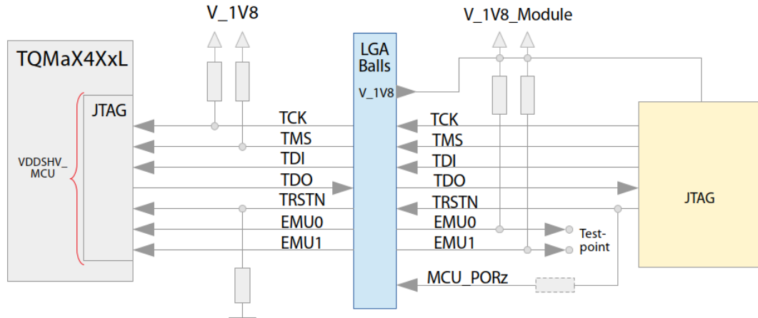
Figure 25: Block diagram JTAG
