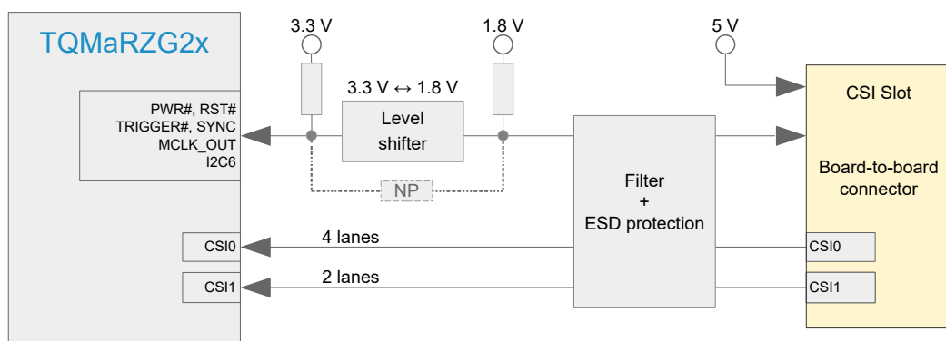
Figure 23: Block diagram CSI
