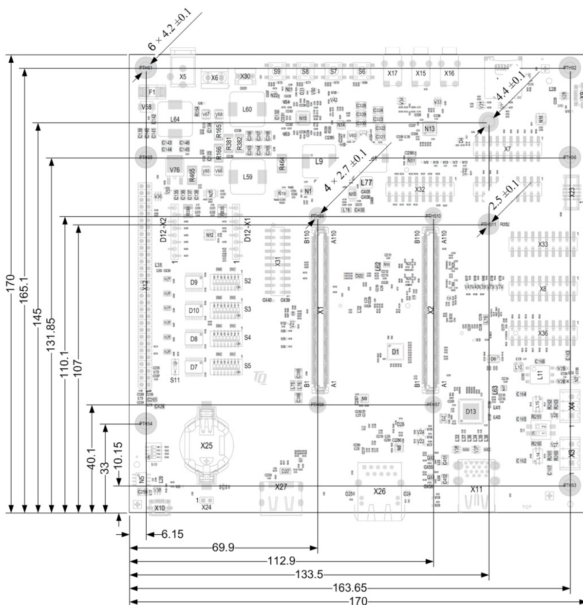
Figure 28: MBaRZG2x dimensions
