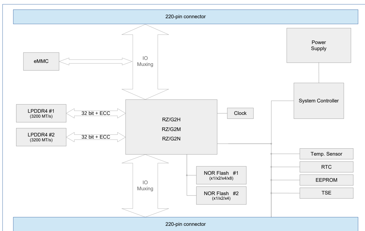
Figure 4: Block diagram TQMaRZG2x
