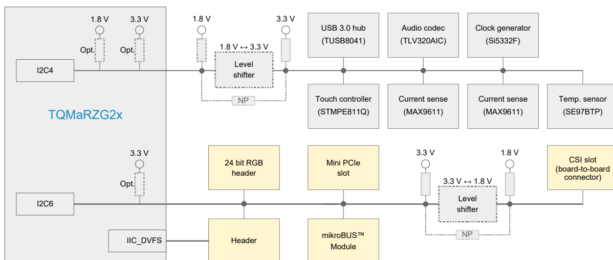
Figure 8: Block diagram I2C bus
