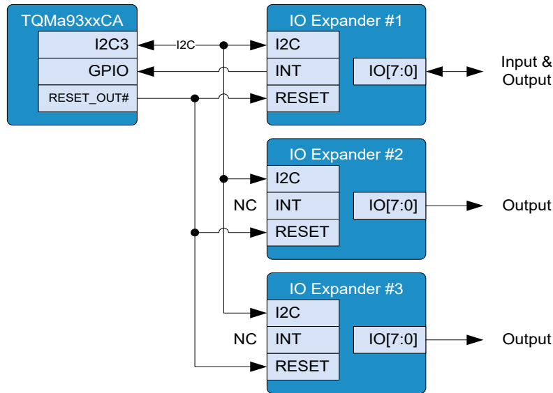
Figure 3: Block diagram GPIO expanders
