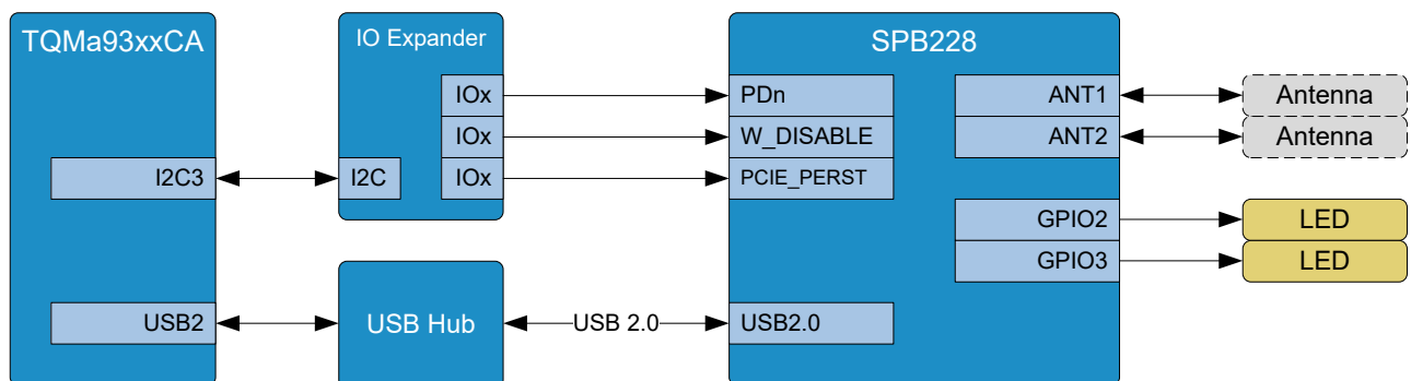
Figure 10: Block diagram WLAN / wireless
