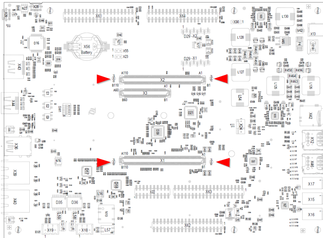
Figure 28: Position of heat sink mounting holes
