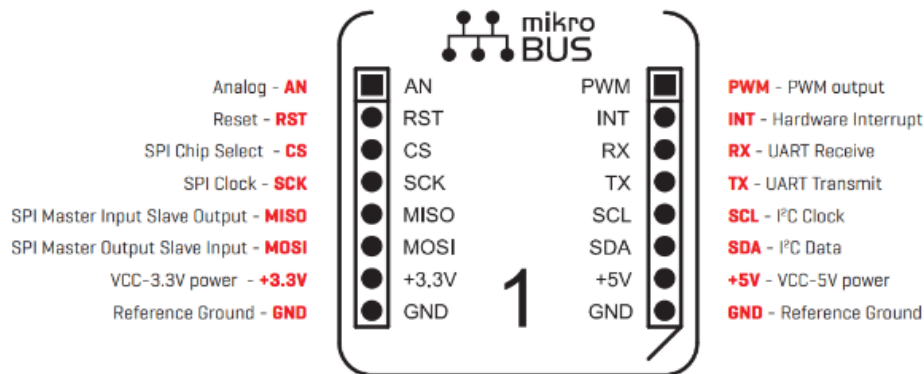
Figure 24: Pinout microbus (source: MikroElektronika)
