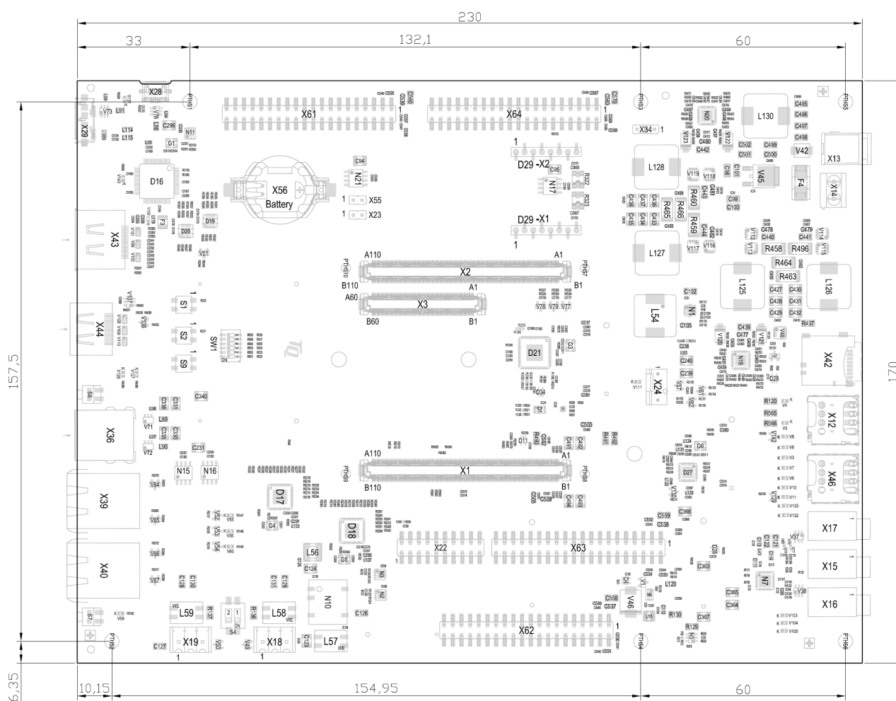
Figure 29: MBa8x dimensions
