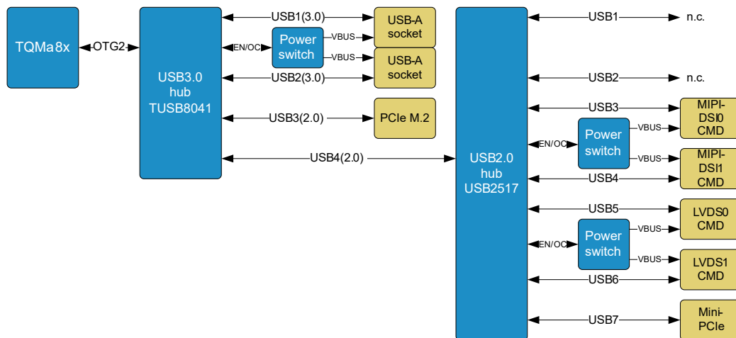
Figure 21: Block diagram USB hub structure of the MBa8x
