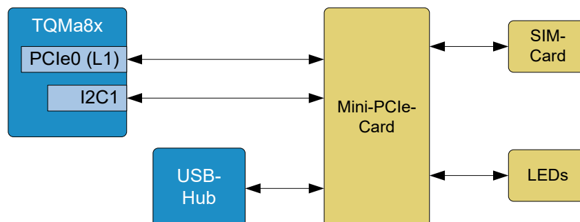
Figure 17: Block diagram Mini-PCIe
