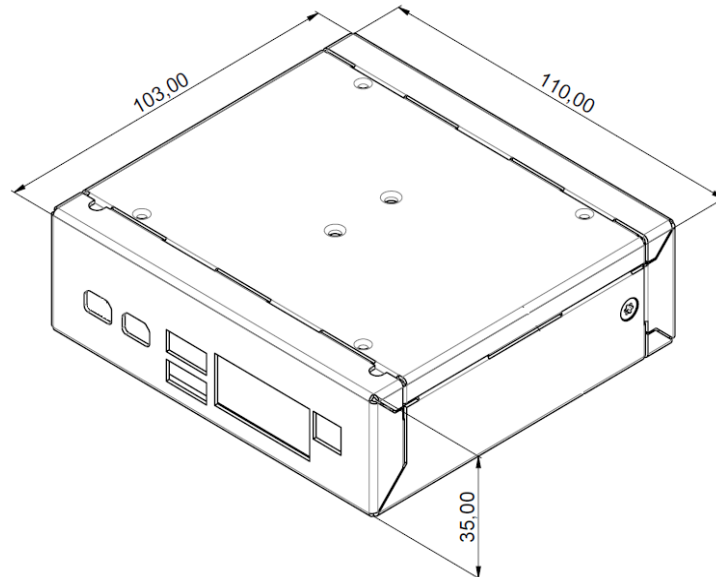
Figure 4: ABox-93xxLA (without connectors), Dimensions (mm), Bottom View
