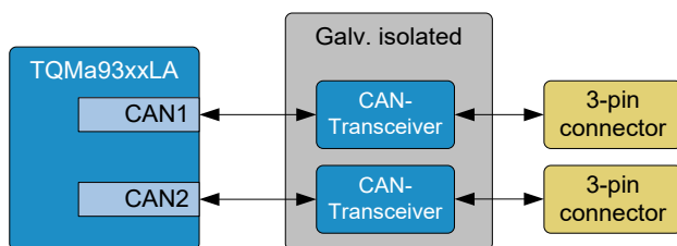
Figure 3: Block diagram CAN
