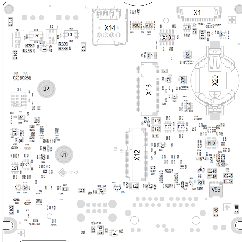
Figure 6: ABox-93xxLA component placement
