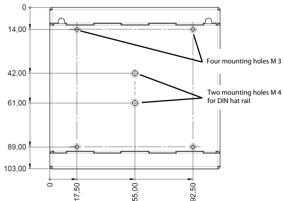
Figure 5: ABox-93xxLA, Dimensions of Mounting Holes (mm), Bottom View
