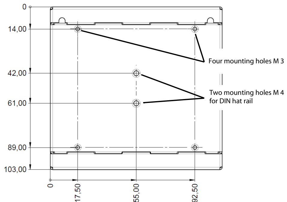
Figure 4: ABox-93xxLA, Dimensions of Mounting Holes (mm), Bottom View
