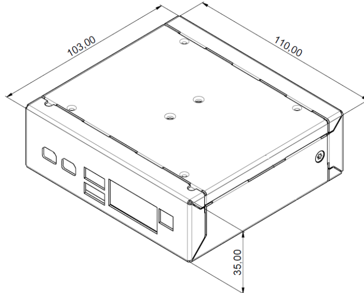
Figure 3: ABox-93xxLA (without connectors), Dimensions (mm), Bottom View
