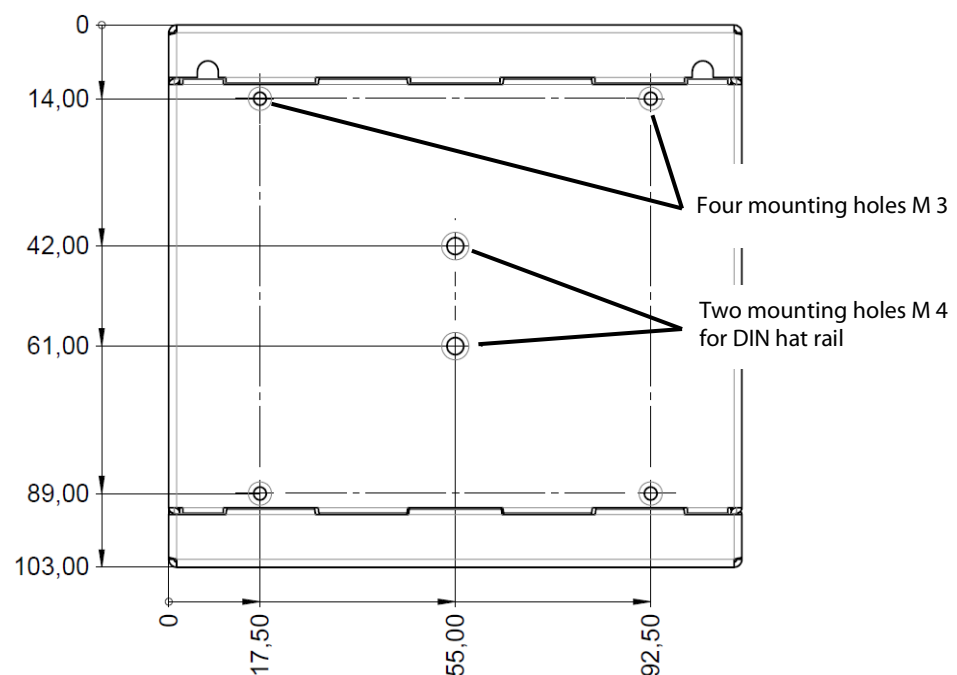
Figure 4: ABox-93xxLA-MINI, Dimensions of Mounting Holes (mm), Bottom View
