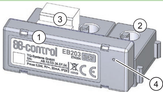
Fig. 1: Items supplied with the Sensorbar, example of EB203
