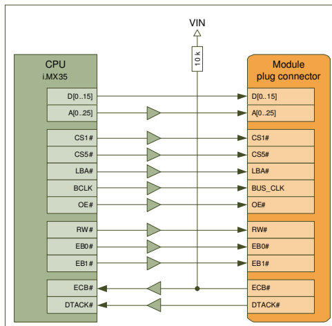
Illustration 3: Interface WEIM bus
