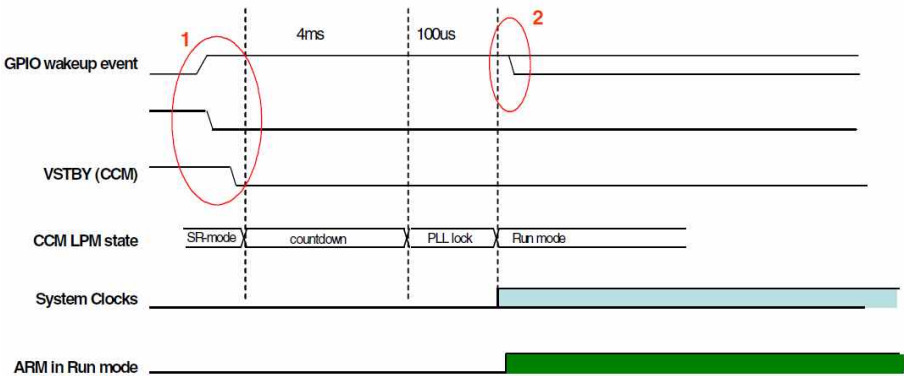
Illustration 15: Timing diagram of a GPIO wakeup interrupt (Source: i.MX35 Reference Manual Rev. 3 )
