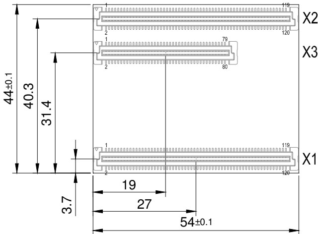
Illustration 17: Overall dimensions (top view through board)
