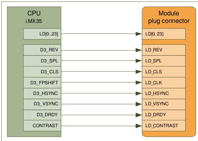
Illustration 4: Interface LCD
