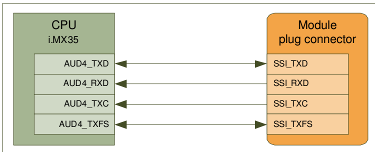
Illustration 14: Interface SSI
