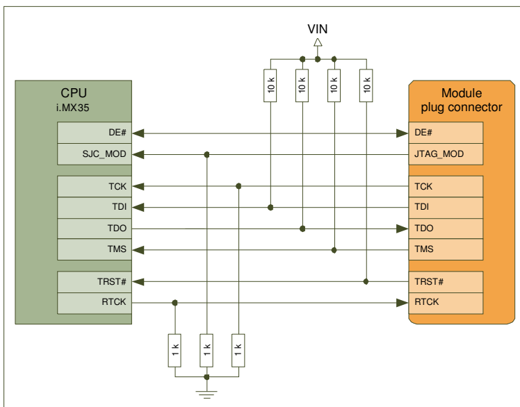
Illustration 16: Interface BDM/JTAG
