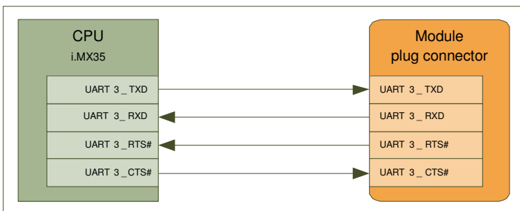
Illustration 12: Interface UART3
