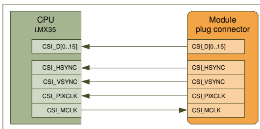
Illustration 5: Interface CSI
