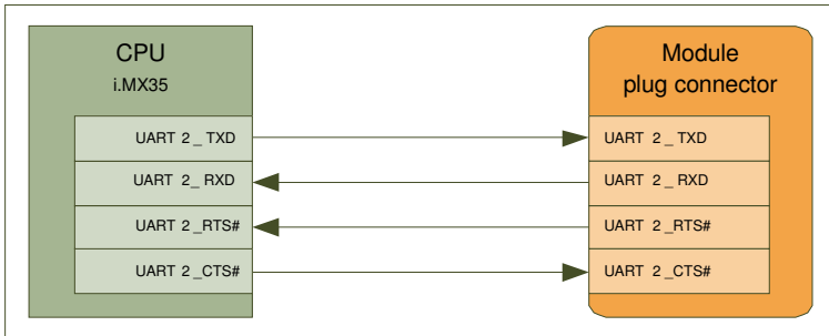
Illustration 11: Interface UART2
