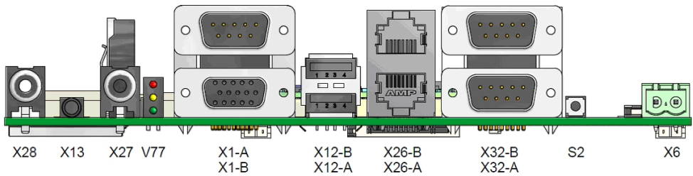
Illustration 2: External interfaces of the STK-MBa35
