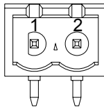
Illustration 25: Wiring of X6 (View on contacts from outside)
