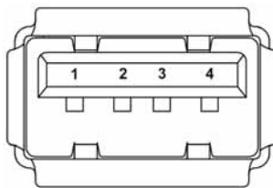
Illustration 21: Wiring of X12-B
