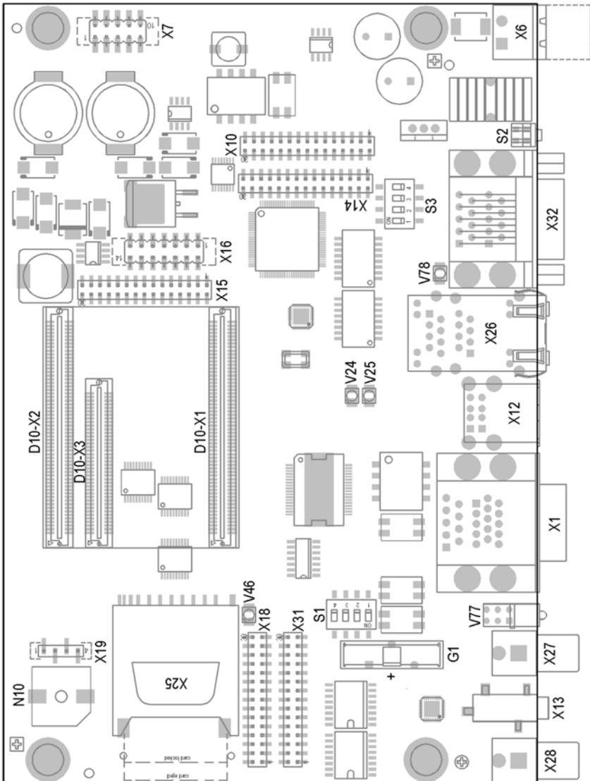
Illustration 39: Top view
