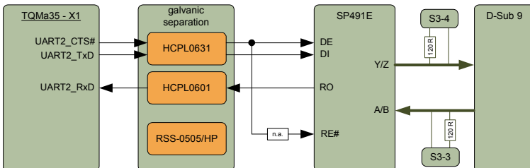
Illustration 5: Block diagram RS485
