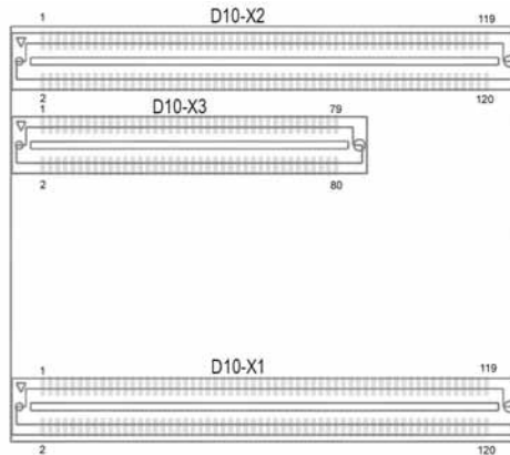
Illustration 34: Wiring of D10
